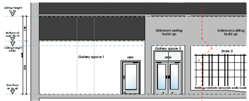
D-D Proposed - Section D-D 1:100
