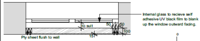
Proposed Infill panel plan 1:20
